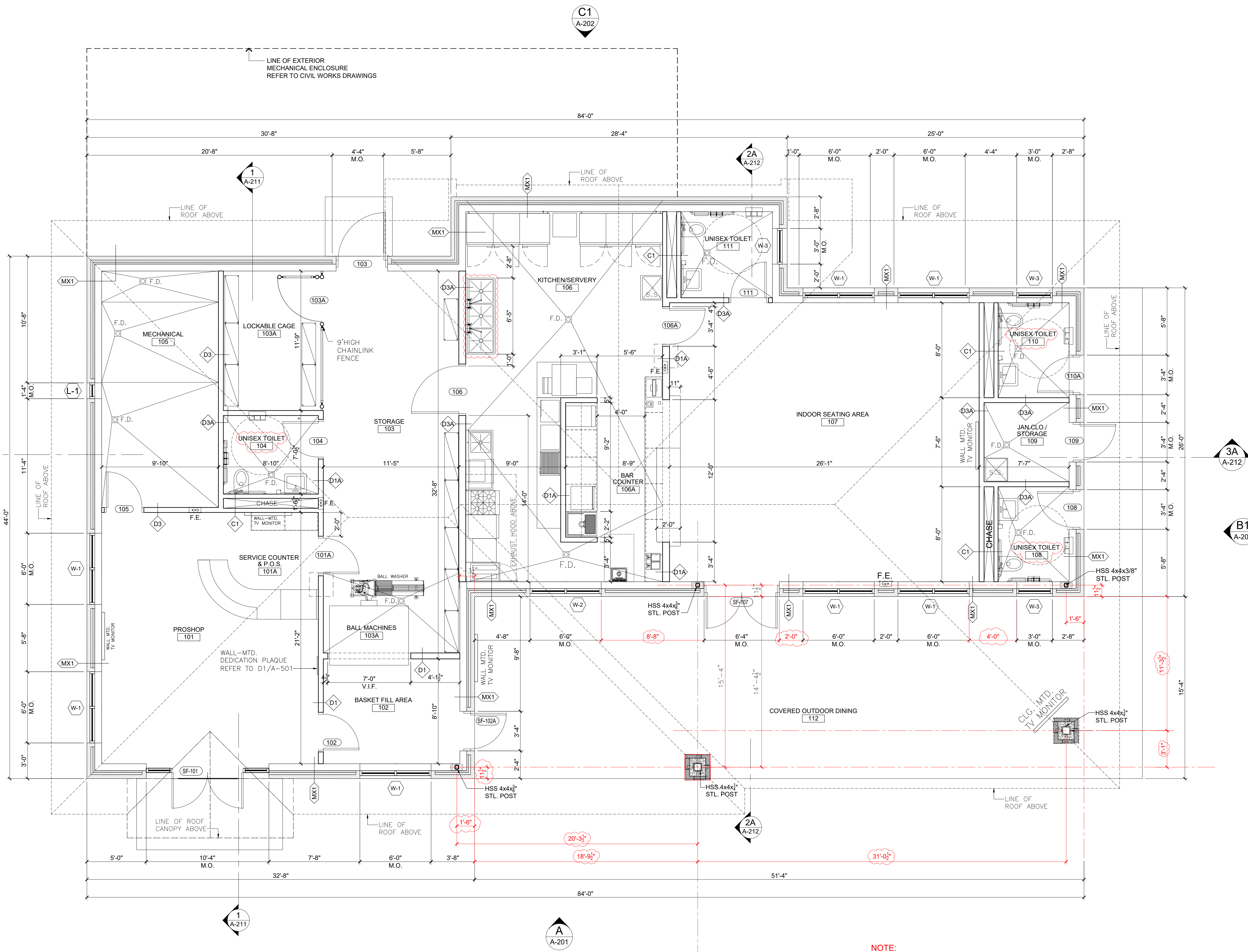
1 CONSTRUCTION PLAN - ALTERNATE BID SCALE: 1/4" = 1' - 0"
